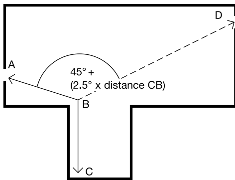
Diagram 15 Travel distance in dead-end condition
