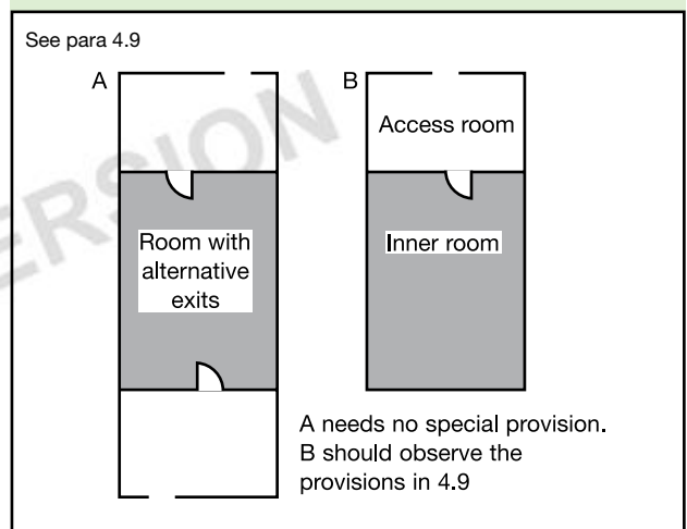
Diagram 17 Inner room and access room
