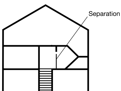
c. Stair to new storey is in space converted and separated from first floor accommodation. New storey open to new stair. New stair separated from original stair at first floor level.
