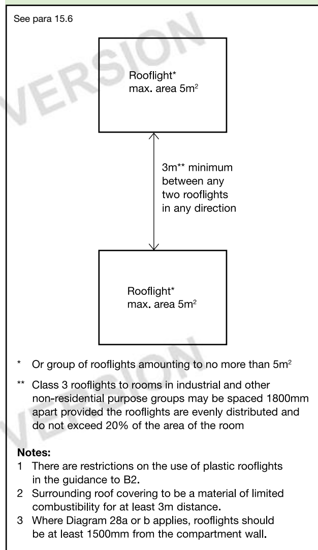
Diagram 47 Limitations on spacing and size of plastic rooflights having a Class 3 or TP(b) lower surface
