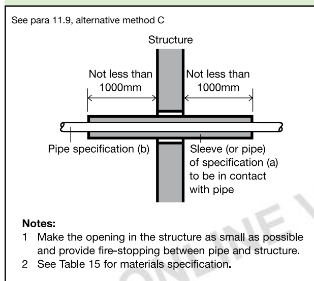
Diagram 37 Pipes penetrating structure
