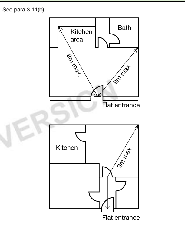
Diagram 8 Flat with restricted travel distance from furthest point to entrance
