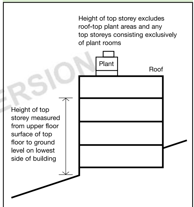
Diagram C5 Height of top storey in building
