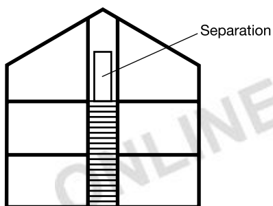
a. Stair to new storey is within existing stairway. Separation of accommodation on new storey from stair is at top level.
