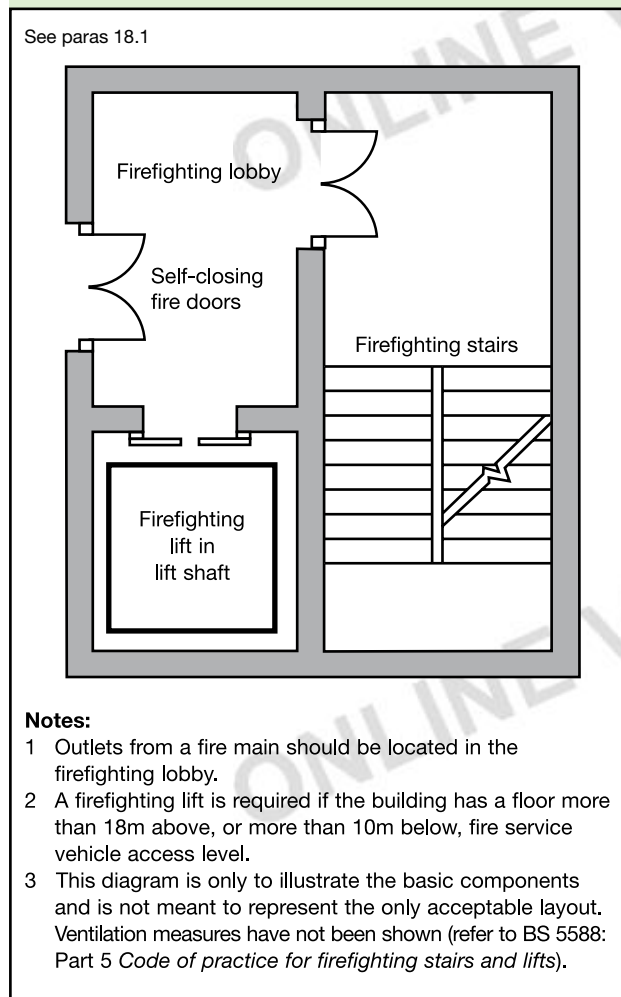
Diagram 52 Components of a firefighting shaft
