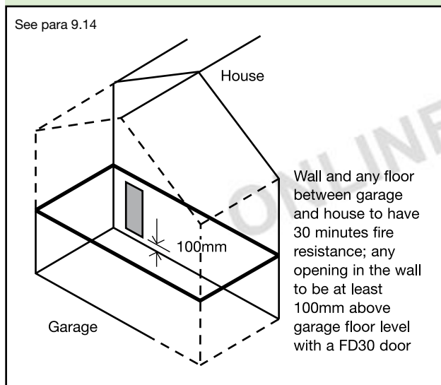
Diagram 25 Separation between garage and dwellinghouse
