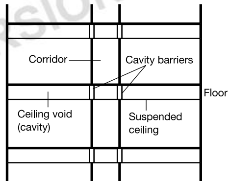
a. SECTION TO SHOW USE OF CAVITY BARRIERS ABOVE THE CORRIDOR ENCLOSURE
