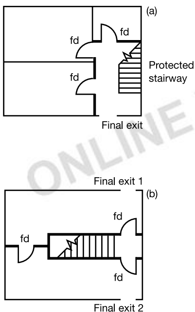
Diagram 3 Alternative arrangements for final exits
