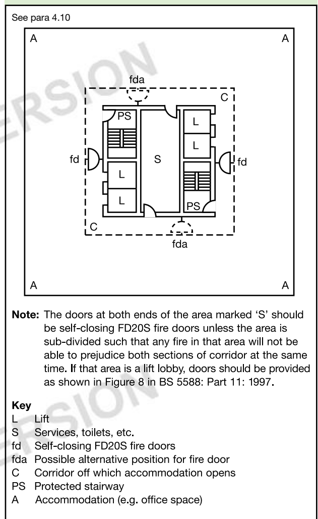
Diagram 18 Exits in a central core
