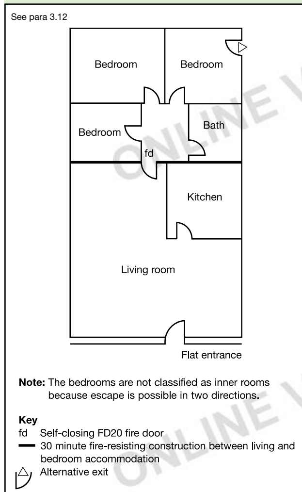
Diagram 9 Flat with an alternative exit, but where all habitable rooms have no direct access to an entrance hall
