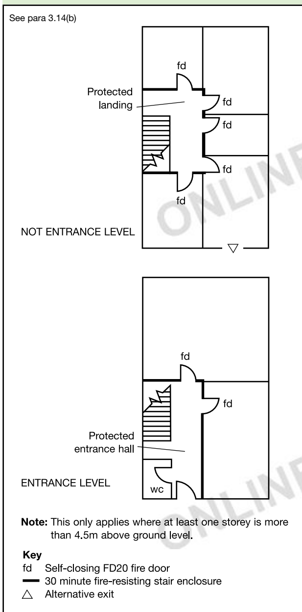
Diagram 11 Maisonnette with protected entrance hall and landing
