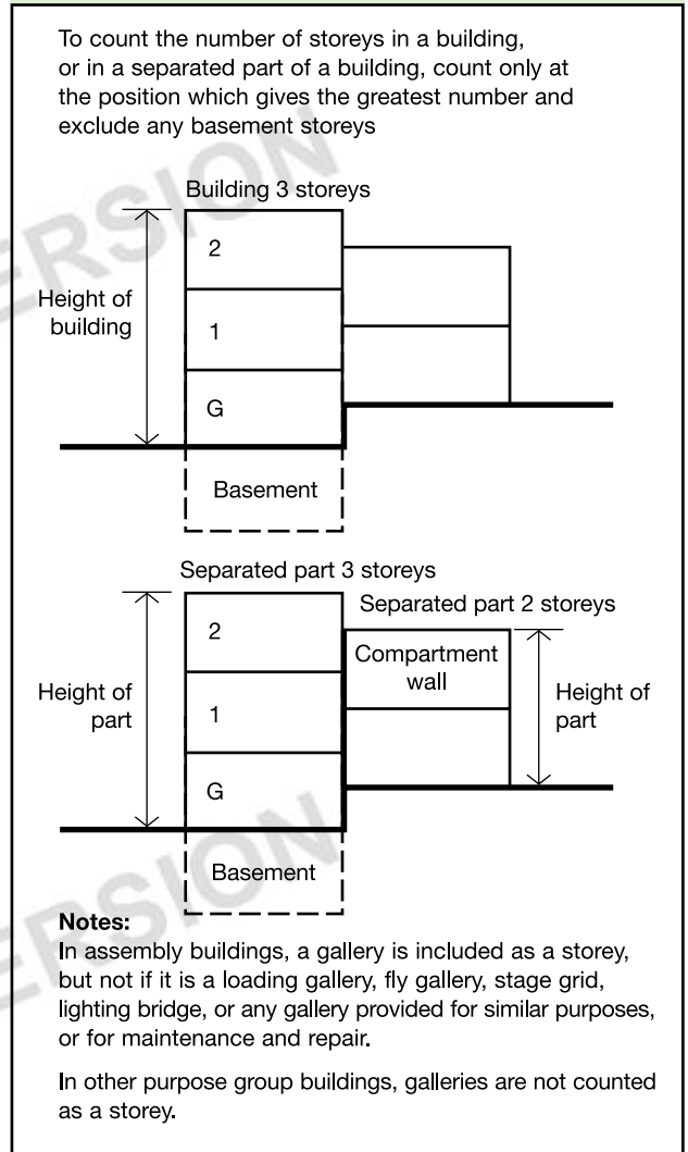
Diagram C4 Number of storeys
