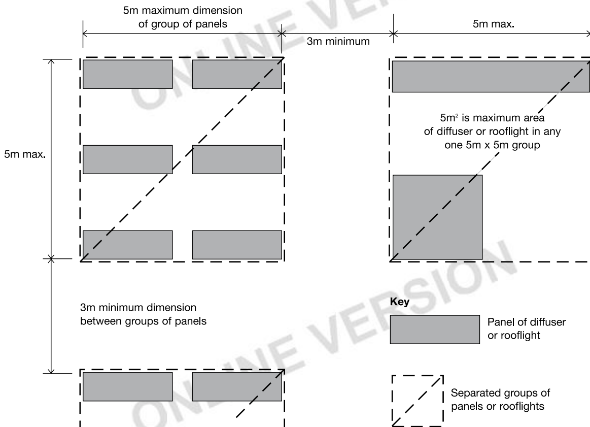
Diagram 24 Layout restrictions on Class 3 plastic rooflights, TP(b) rooflights and TP(b) lighting diffusers
