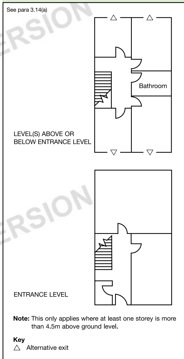
Diagram 10 Maisonette with alternative exits from each habitable room, except at entrance level
