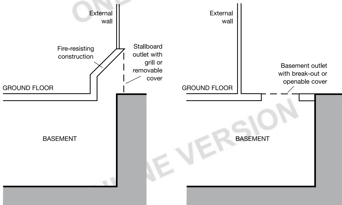
Diagram 53 Fire-resisting construction for smoke outlet shafts
