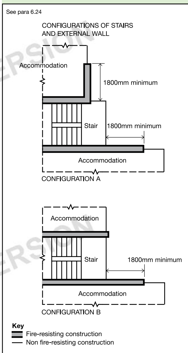
Diagram 21 External protection to protected stairways
