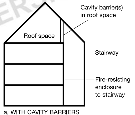
a. WITH CAVITY BARRIERS
