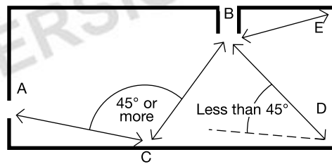
Diagram 16 Alternative escape routes
