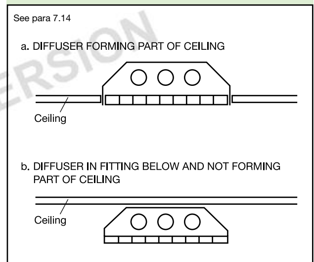
Diagram 23 Lighting diffuser in relation to ceiling
