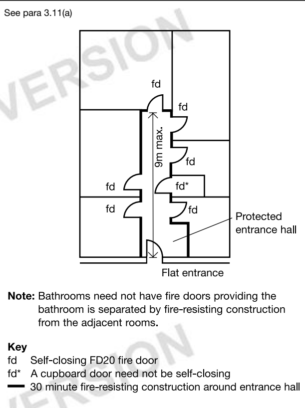
Diagram 7 Flat where all habitable rooms have direct access to an entrance hall
